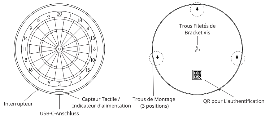
GRANBOARD132 FRONT
